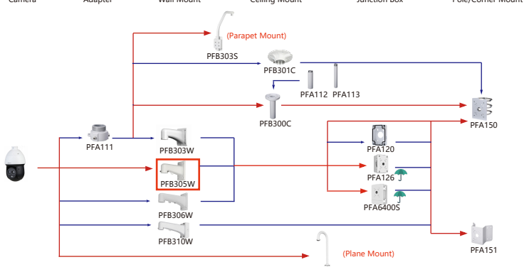
Camera Adapter Wall Mount Ceiling Mount Junction Box Pole/Corner Mount
