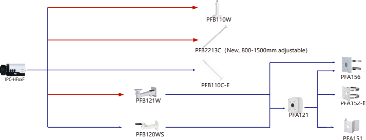
Selection of Lens(610 Series)
