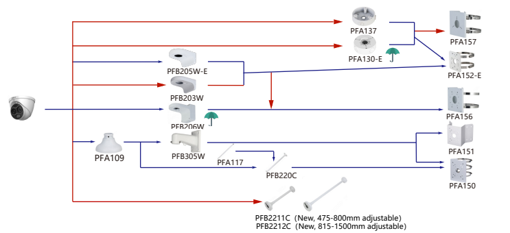
Camera Adapter Wall Mount Ceiling Mount Junction Box Pole/Corner Mount
