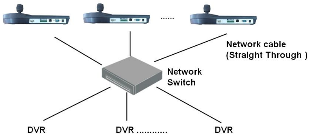
Appendix Figure 1-2 Connection through switch
