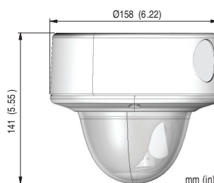
Surface-mount dimensions (with separately available VDA-455SMB-IP)
