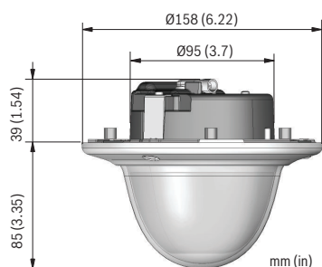
Flush-mount dimensions
