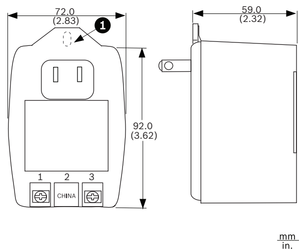
UPA-2430-60 Power Supply
