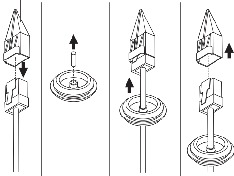
Cap Installer
