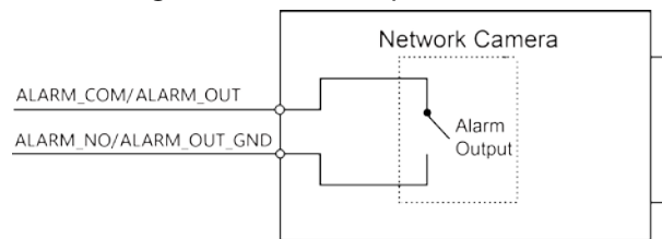
Figure 1-3 Alarm output
