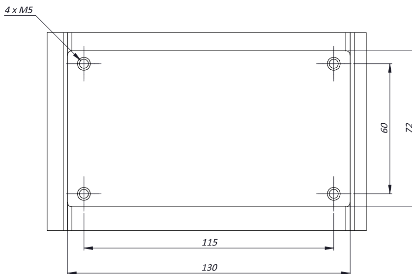
MOUNTING PATTERN
