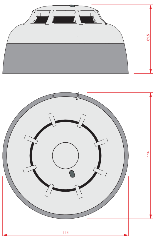
Air2-FD100 - dimensions
