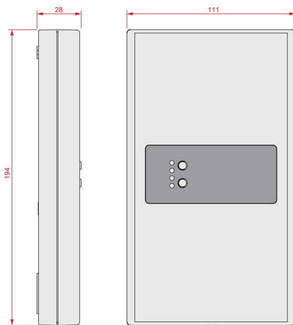
Nexus/3GP - dimensions
