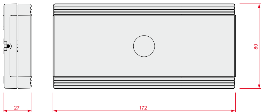
IB200/A - dimensions
