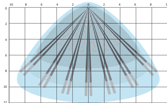
Air2-QDTP200W – Top view
