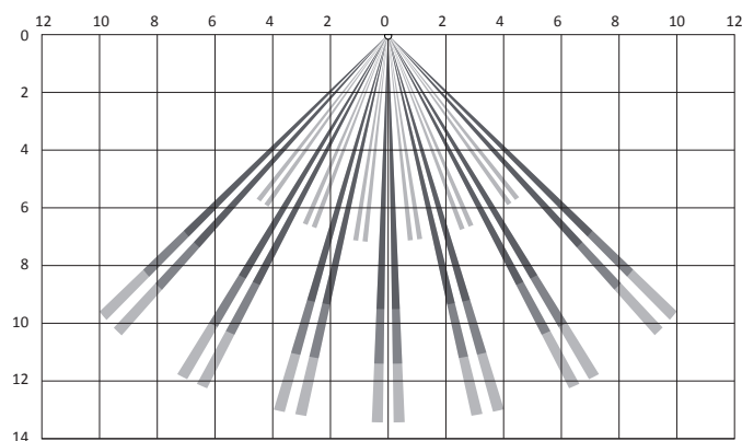
Air2-QIRP200W – Top view
