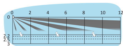
Air2-QDTP200W – Side view
