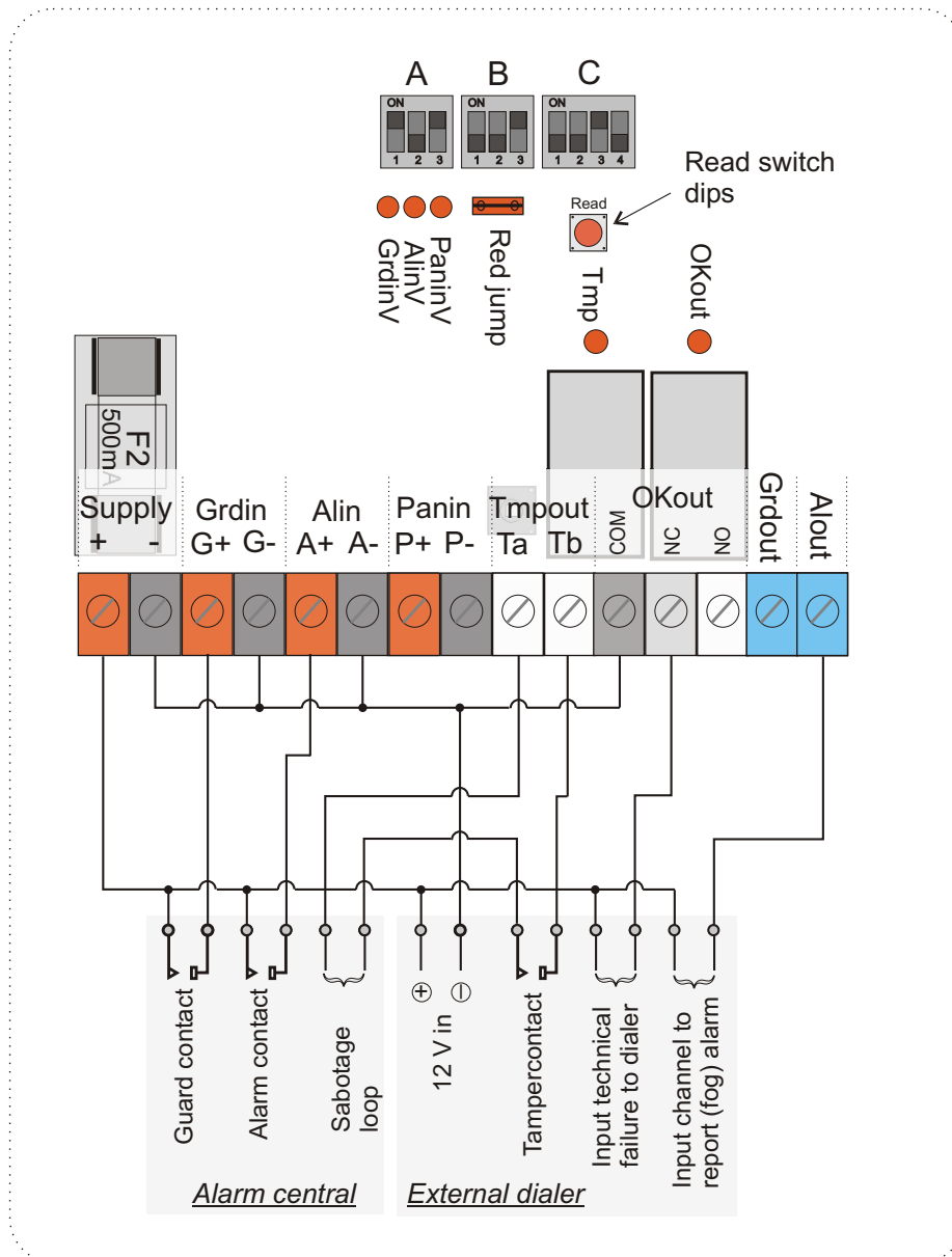
Diagram 3: Alarm system with relay outputs and external dialer to report a technical failure and alarm.
