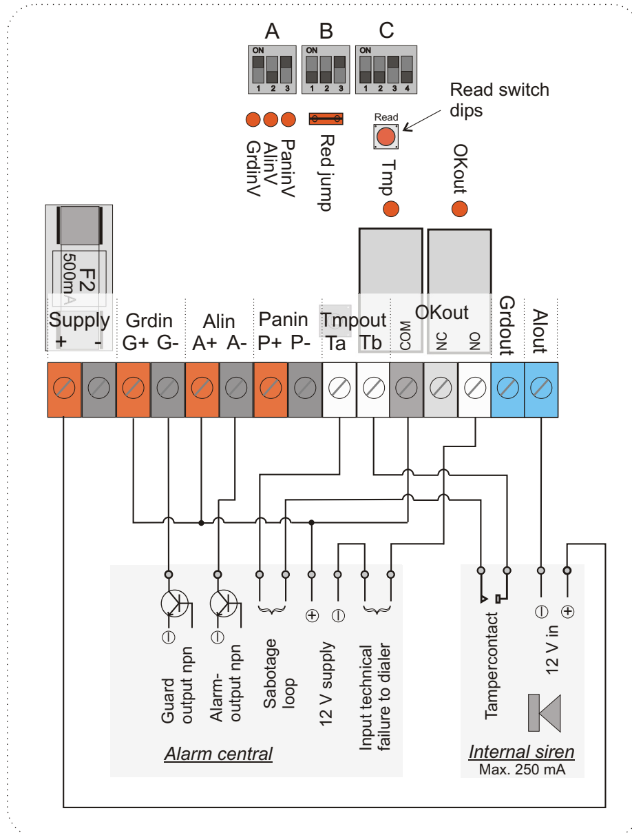
Diagram 1: Alarm system with npn- outputs, technical input and BANDIT -controlled internal siren 12V / max. 250 mA
