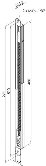
180° DLMC390
