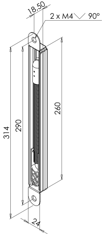
90° DLMC170
