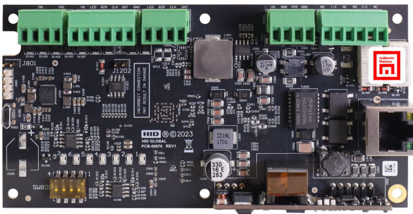
HID Mercury Security MP1501 PoE+ Edge-capable Intelligent Controller
