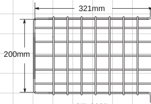
STI-9625 Side View
