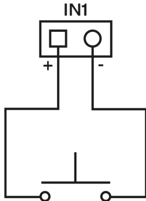
Wiring diagram of IN1 terminals in active mode
