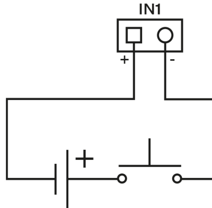
Wiring diagram of IN1 terminals in passive mode
