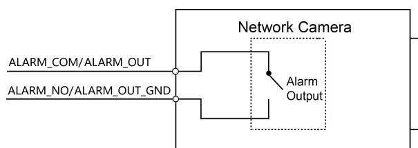
Figure 1-3 Alarm output
