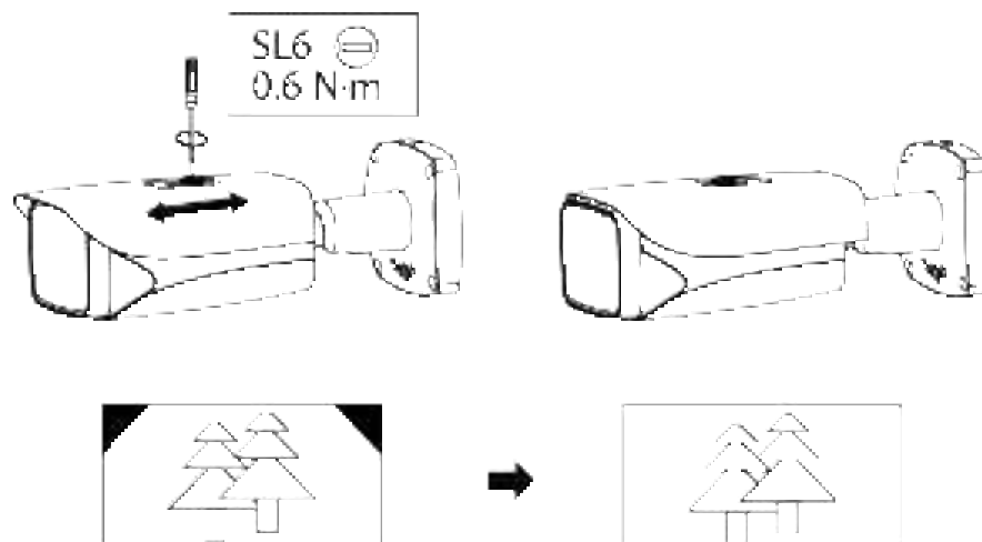
Figure 3-7 Adjust sunshield
