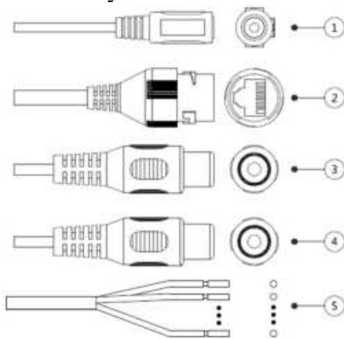
Figure 1-1 Cables
