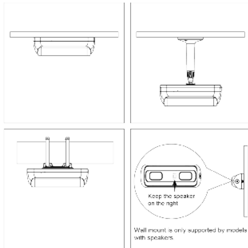
Figure 3-3 Installation method
