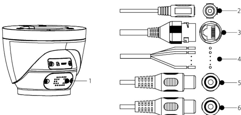
Figure 1-1 Structure components
