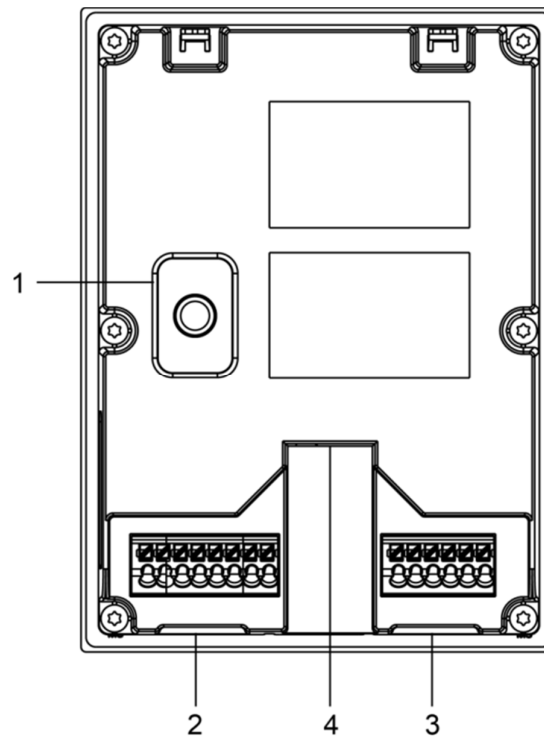
Figure 2-5 Rear panel
