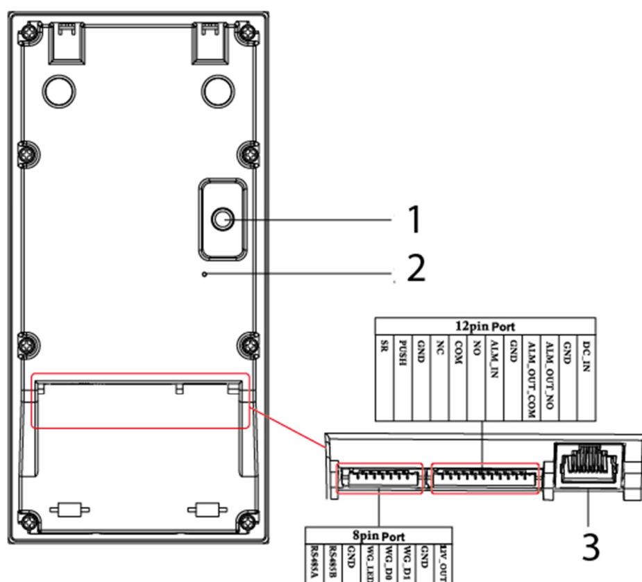
Figure 2-13 VTO3221E-P
