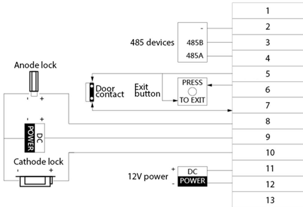
Figure 2-8 Cable connection
