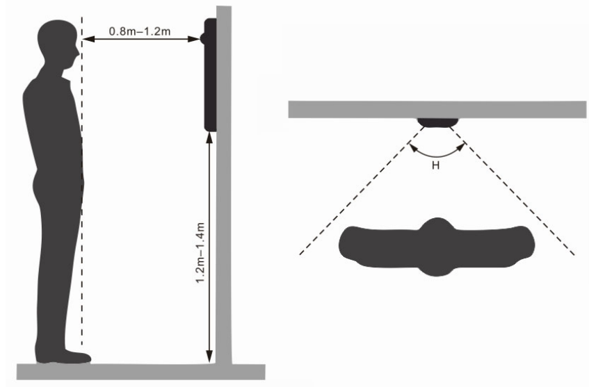
Figure 3-1 Installation position
