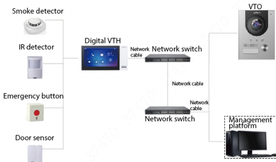
Figure 1-1 Network diagram
