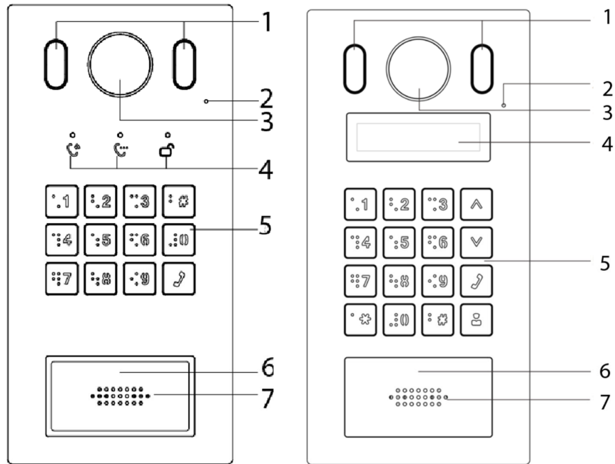
Figure 2-12 VTO3221E-P/VTO6221E-P
