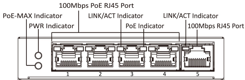
Figure 1-1 DS-3E1105P Series
