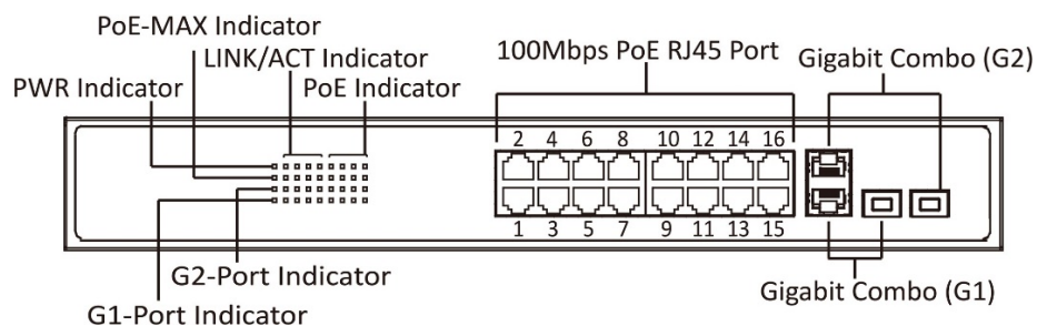
Figure 1-2 DS-3E1318P Series
