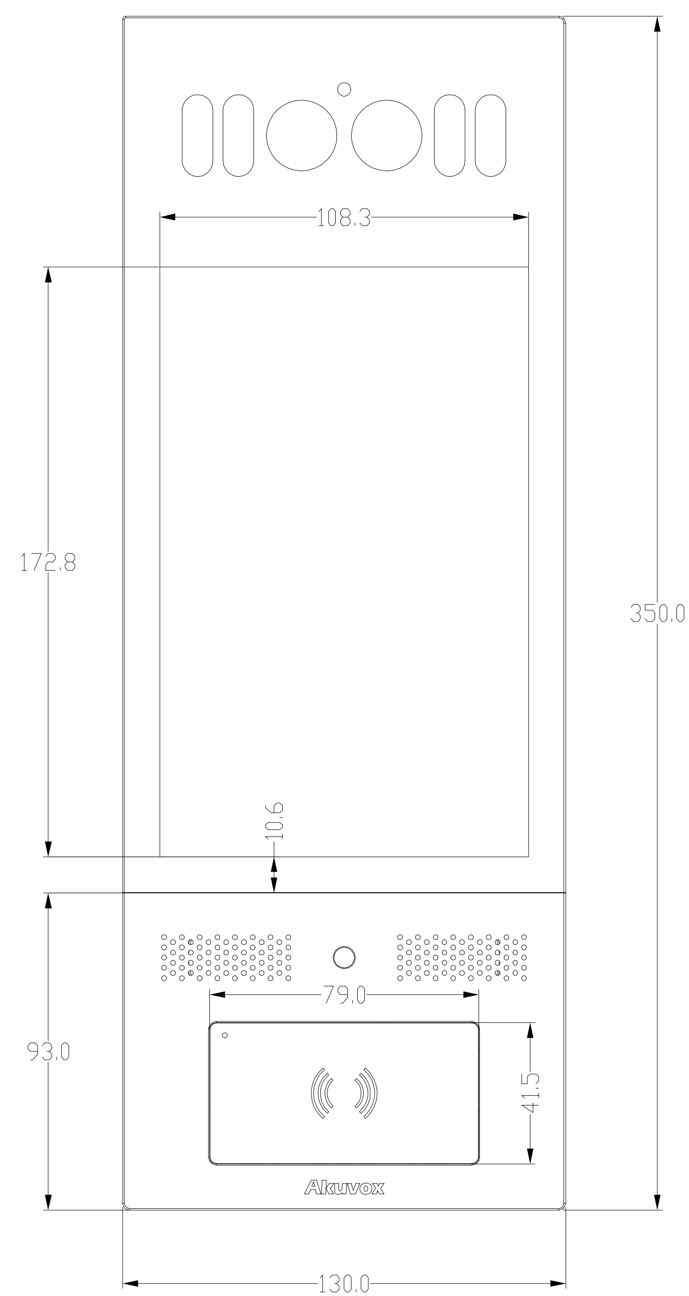
1 FRONT VIEW
